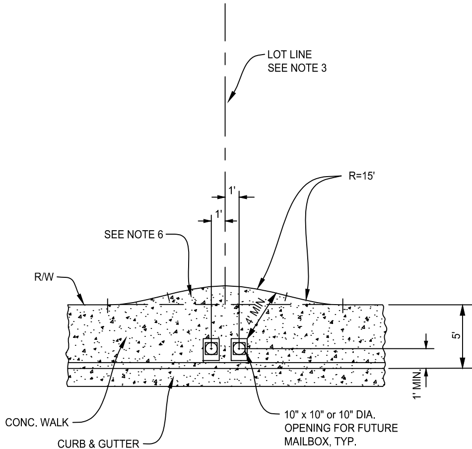
MAILBOX PEDESTAL OPENING(S) DETAIL NOT TO SCALE
