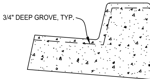
CURB & GUTTER
