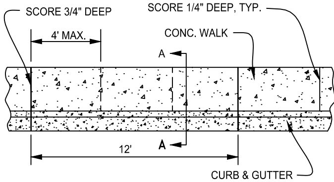
MONOLITHIC SIDEWALK
