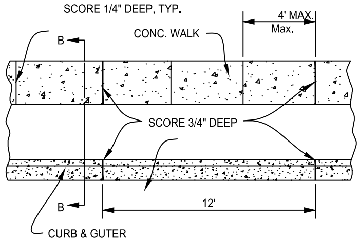
DETACHED SIDEWALK
