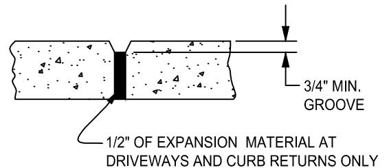
SIDEWALK
