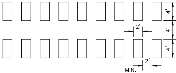
DETAIL - TRIPLE FOUR NOT TO SCALE
