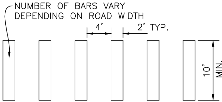
DETAIL - CONTINENTAL NOT TO SCALE
