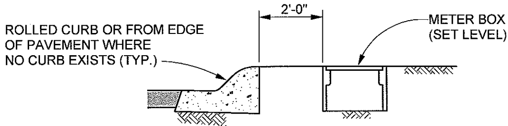
CASE III NO SIDEWALK
