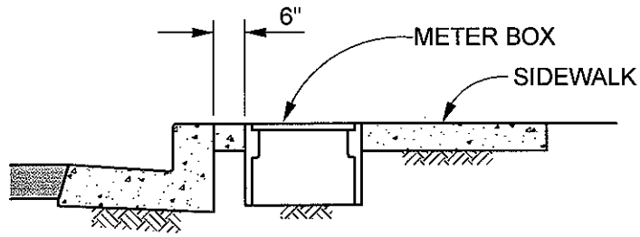
CASE II ATTACHED SIDEWALK
