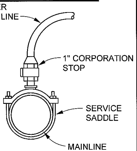
1" COMBINATION AIR RELEASE AND VACUUM VALVE ASSEMBLY
