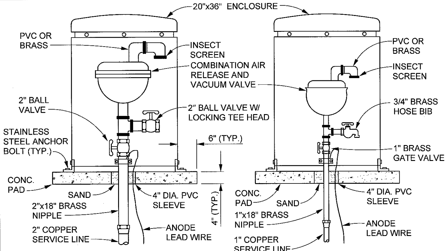
2" COMBINATION AIR RELEASE AND VACUUM VALVE ASSEMBLY
