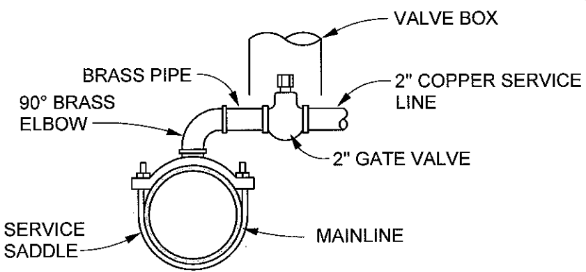
CONNECTION AT HIGH POINT ON WATER MAIN
