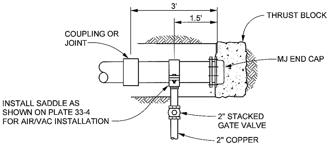
END OF MAIN LOCATION PLAN VIEW
