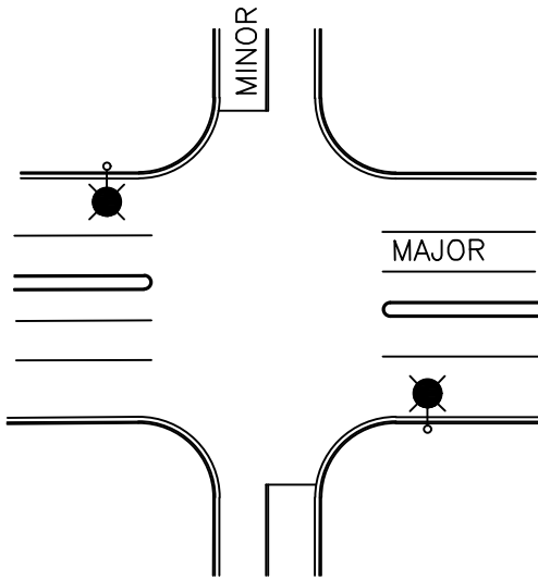
INTERSECTION WITH 2-LANE STREET NOT TO SCALE
