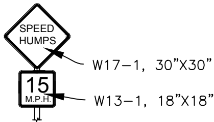
SIGN DETAIL NOT TO SCALE
