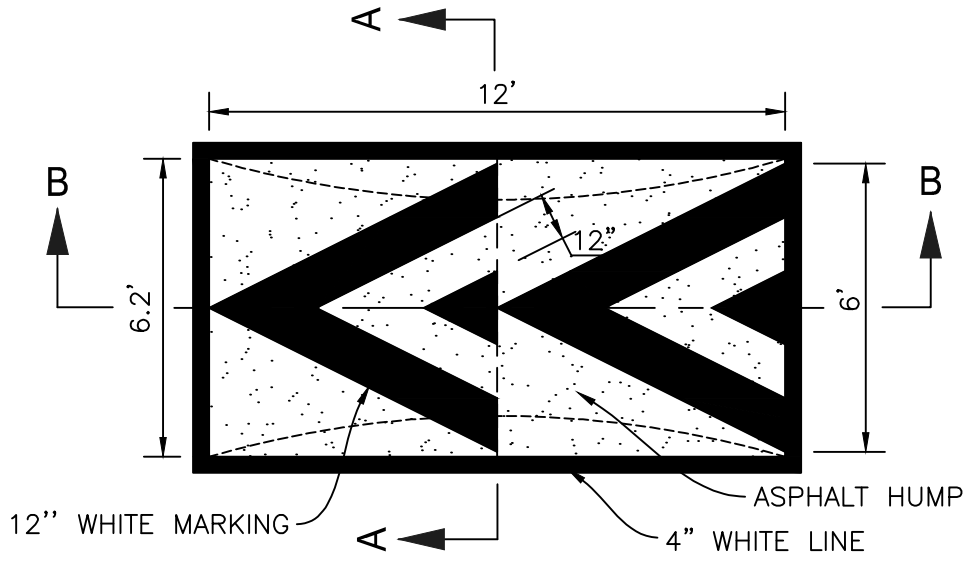
SPEED CUSHION DETAIL SCALE: 1" = 4'
