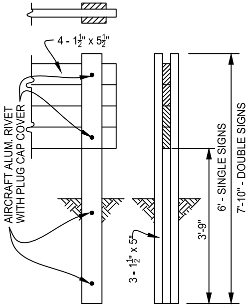
POST DETAIL NOT TO SCALE
