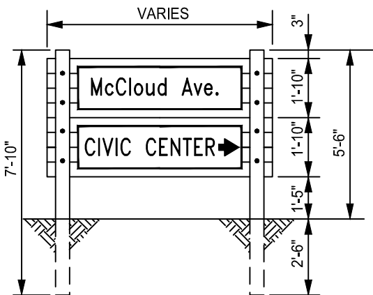
DOUBLE SIGN DETAIL NOT TO SCALE
