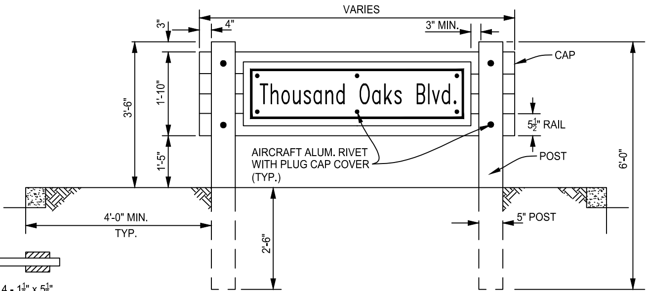
SINGLE SIGN DETAIL NOT TO SCALE
