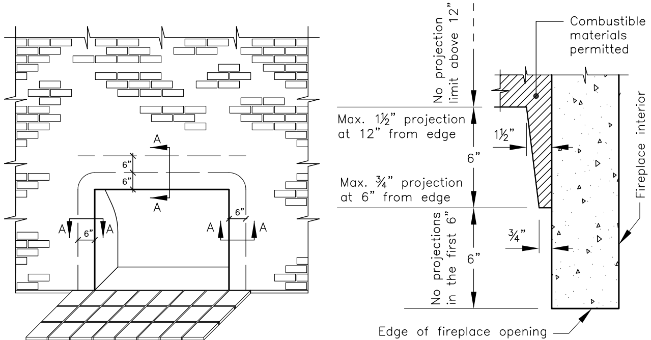
Fireplace Front View
